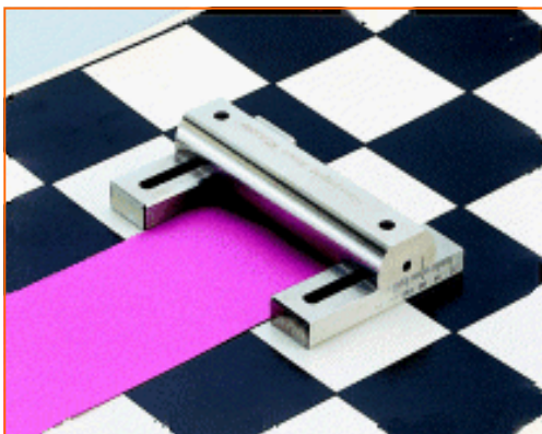
Elcometer 3525 & 3530 Adjustable Baker Film Applicator
